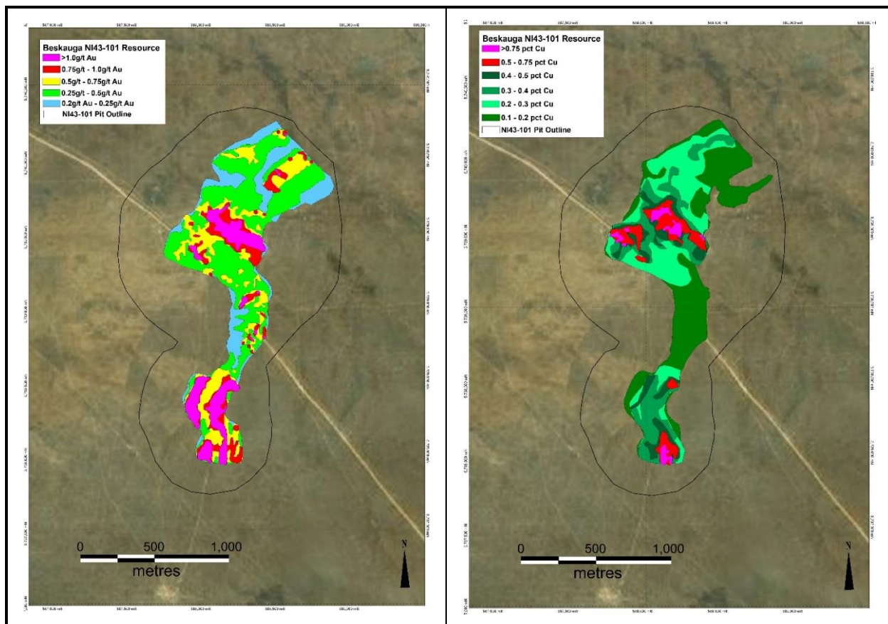
Figure 1. Surface projection of the Beskauga deposit showing the gold and the copper cut-offs. Also shown is the outline of the Lerch-Grossman conceptual pit.
